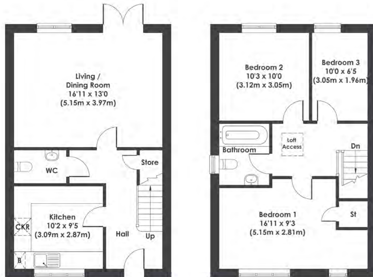
GROUND FLOOR
