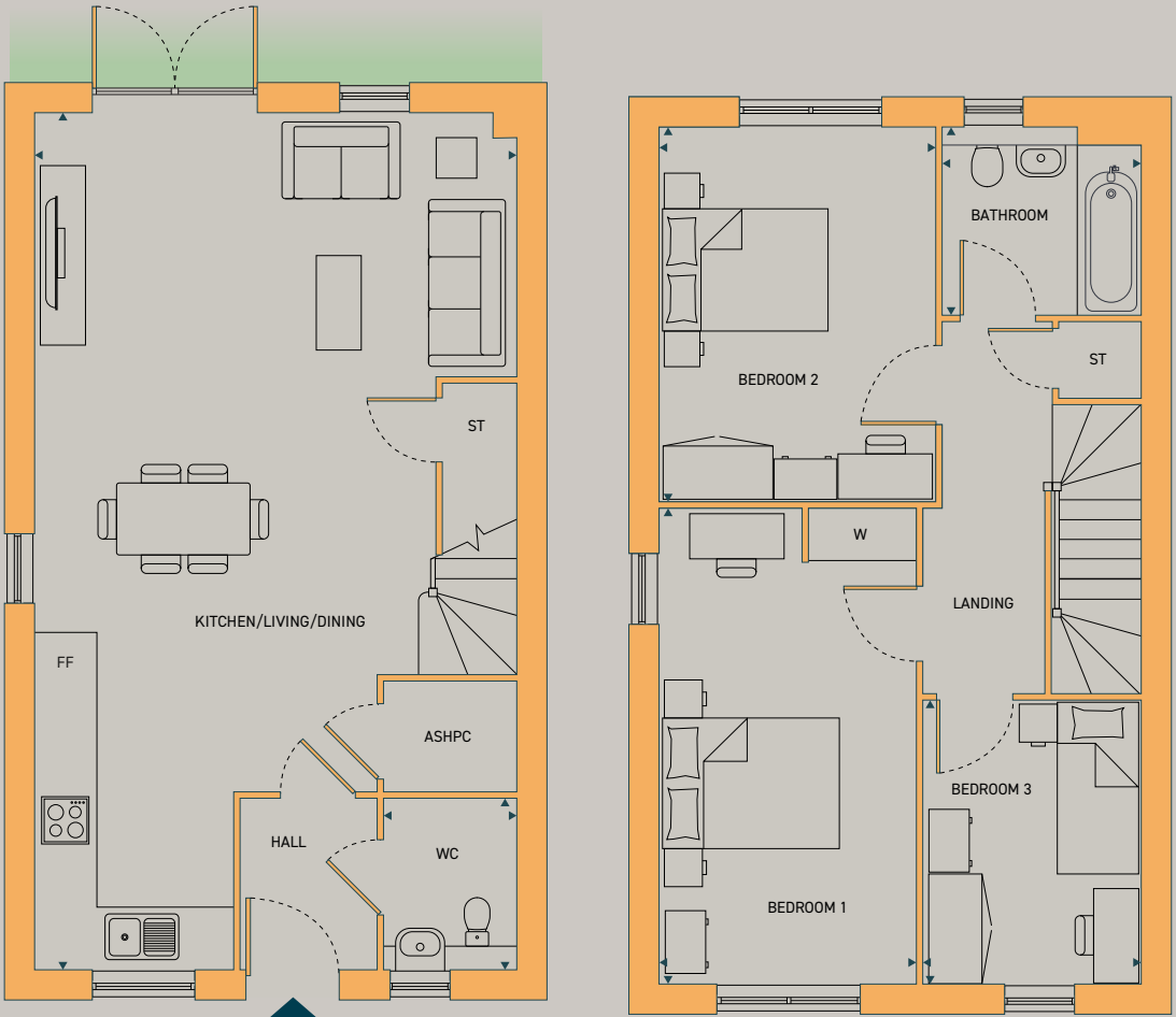
GROUND FLOOR
