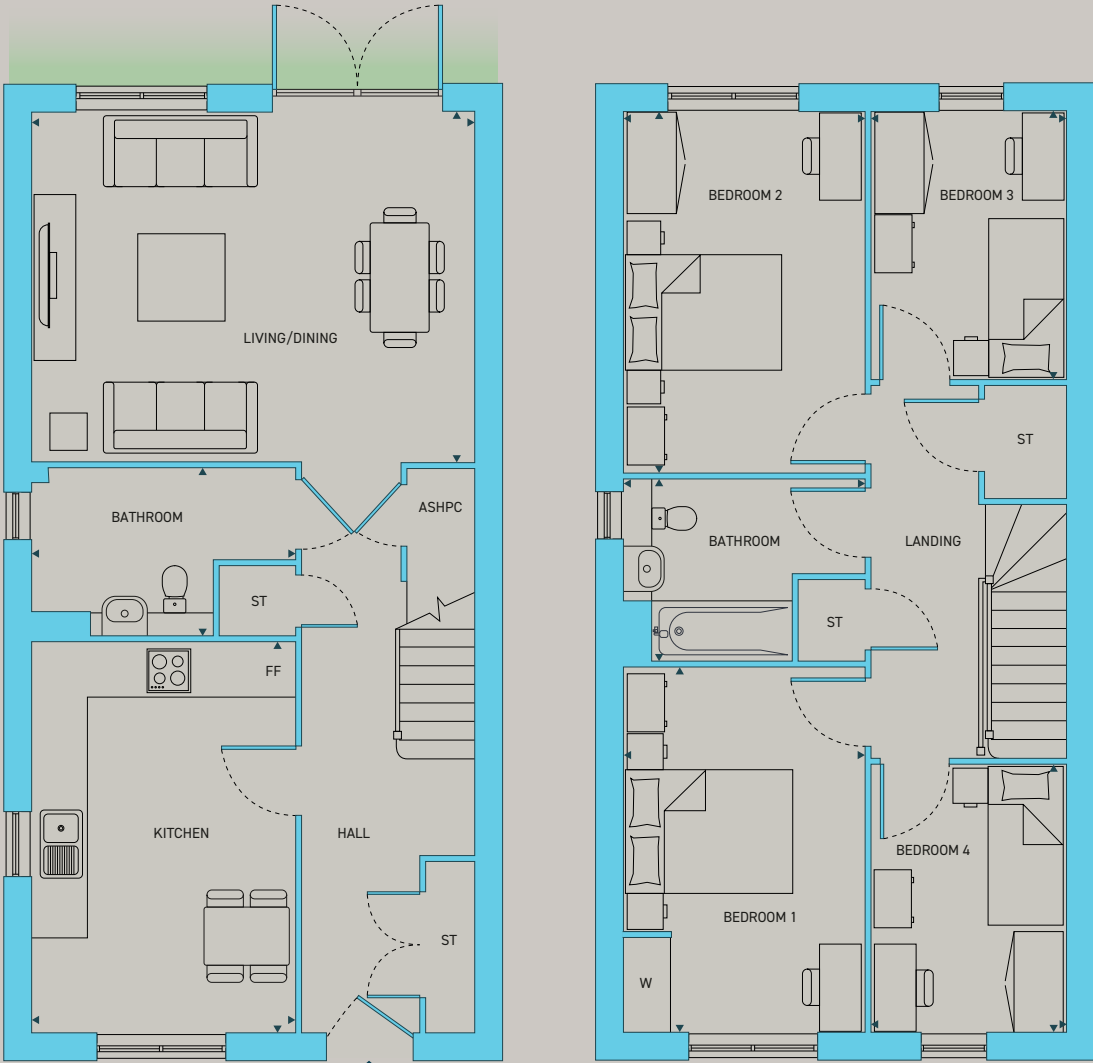
GROUND FLOOR
