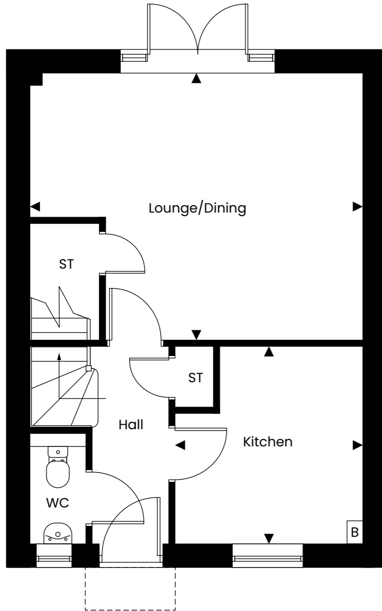
Ground Floor
