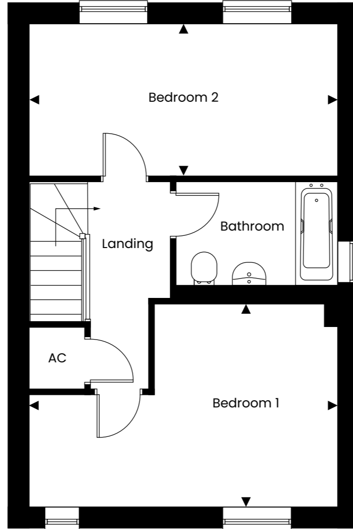
First Floor
