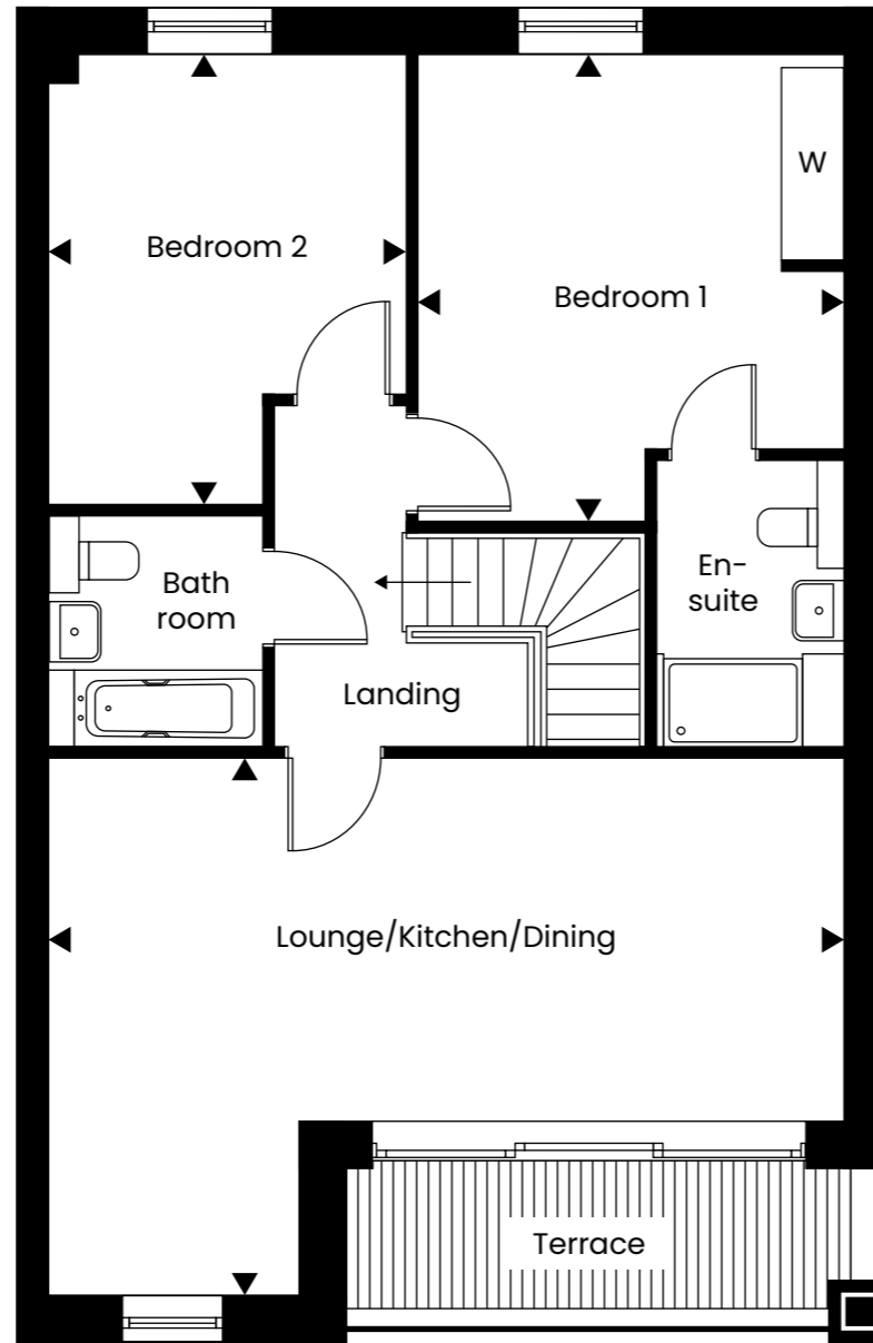
First Floor
