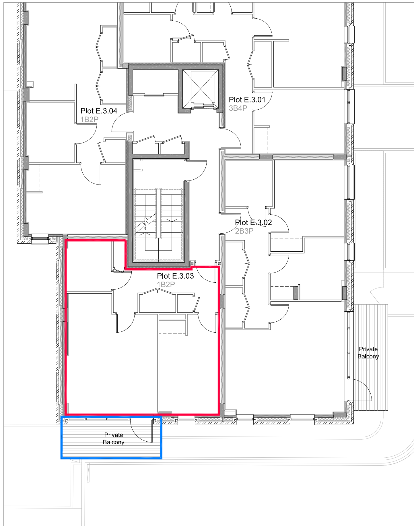
THIRD FLOOR PLAN, PLOT E.3.03
