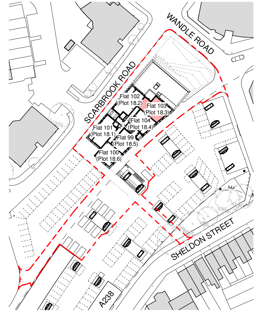
N Flat 103 (Plot 18.3) Eighteenth Floor Scale 1:1000 @ A3
