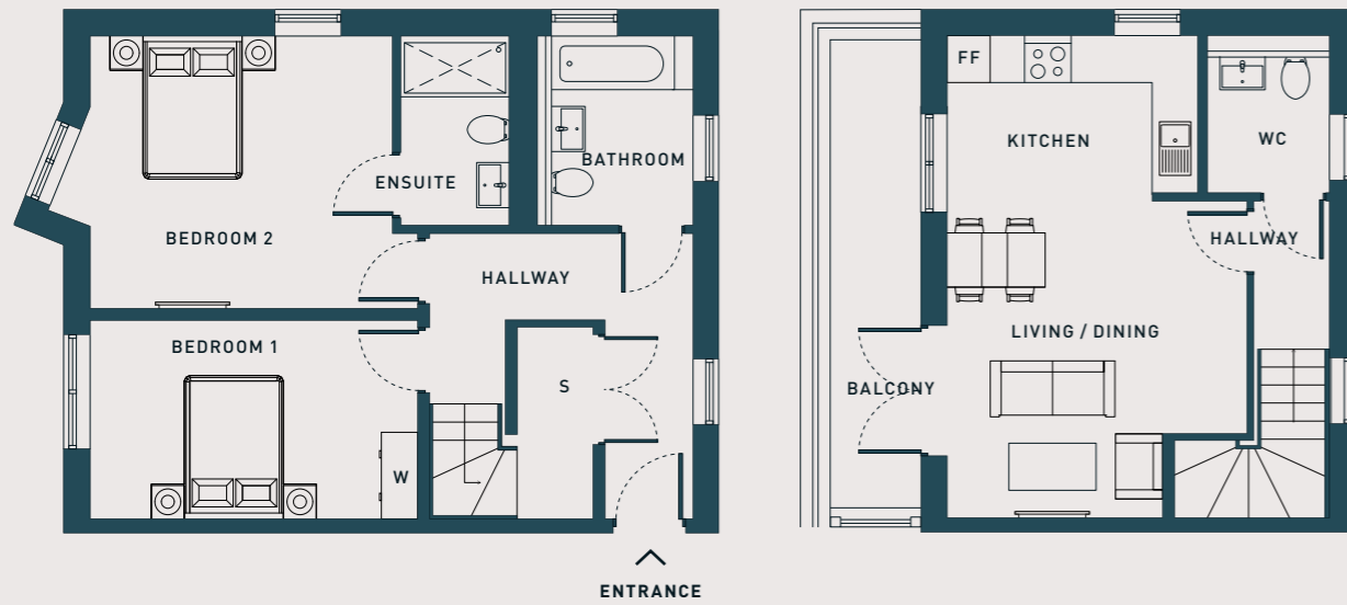
FIFTH FLOOR
