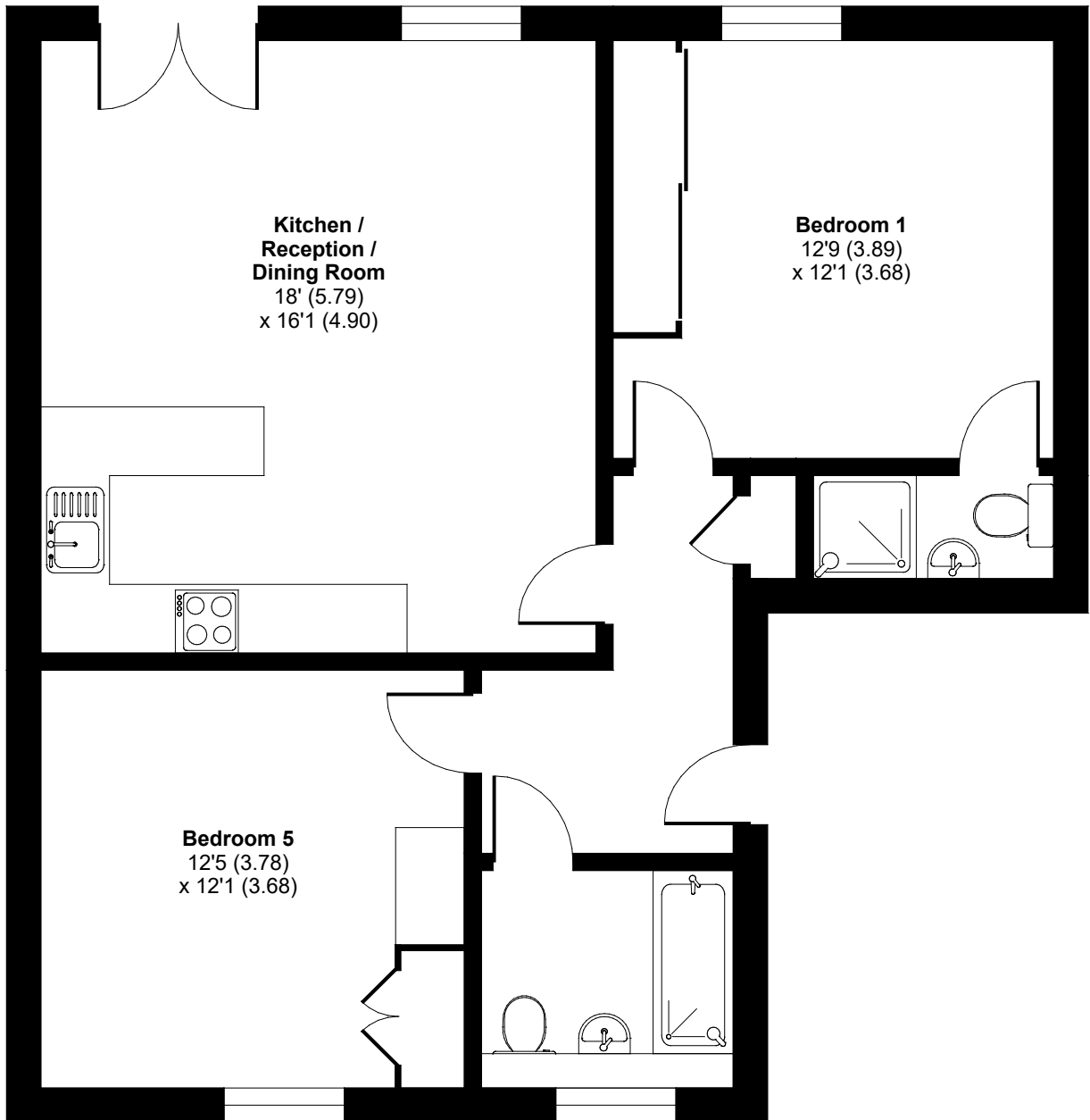
GROUND FLOOR
