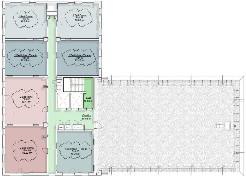
Floor plan – 7 th & 8 th Floor
