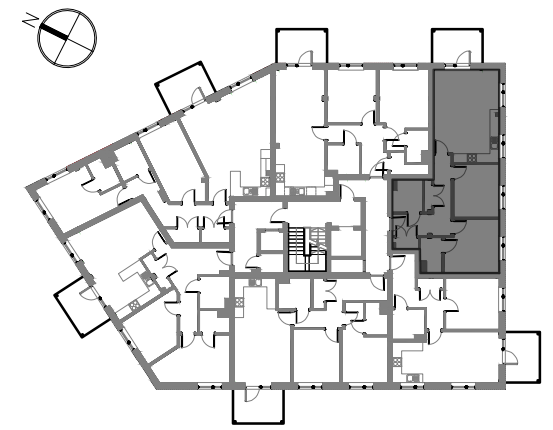
SECOND FLOOR PLAN SCALE 1:500
