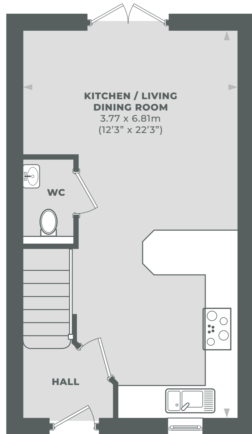
GROUND FLOOR
