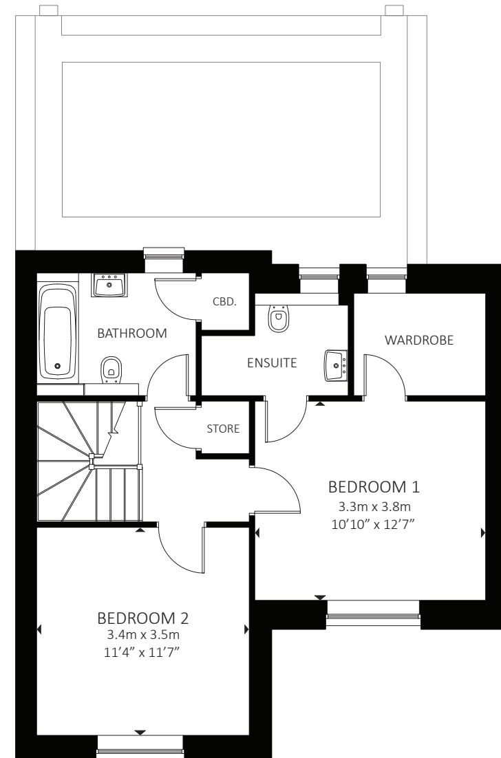
1st Floor PLOT 10
