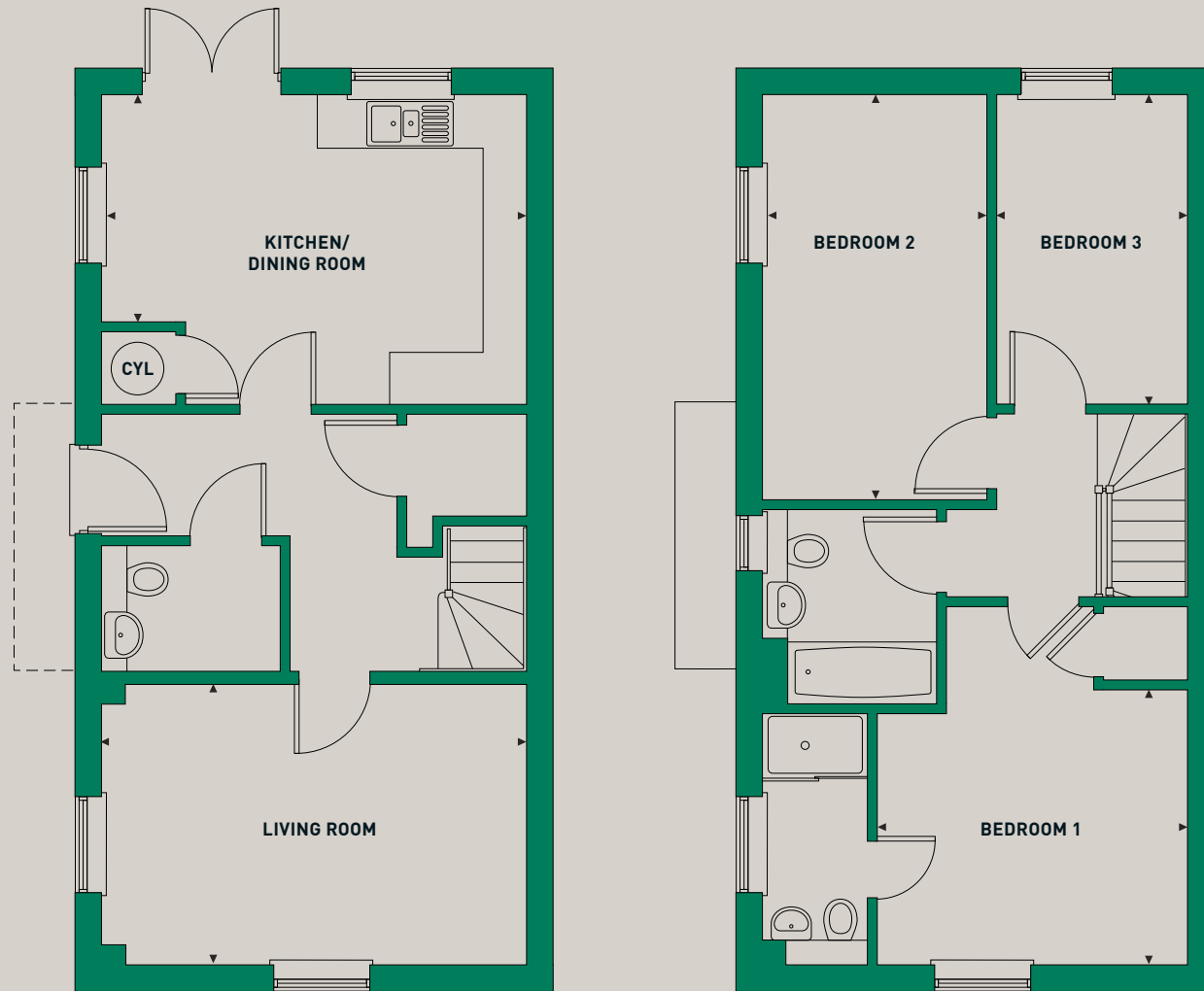
GROUND FLOOR
