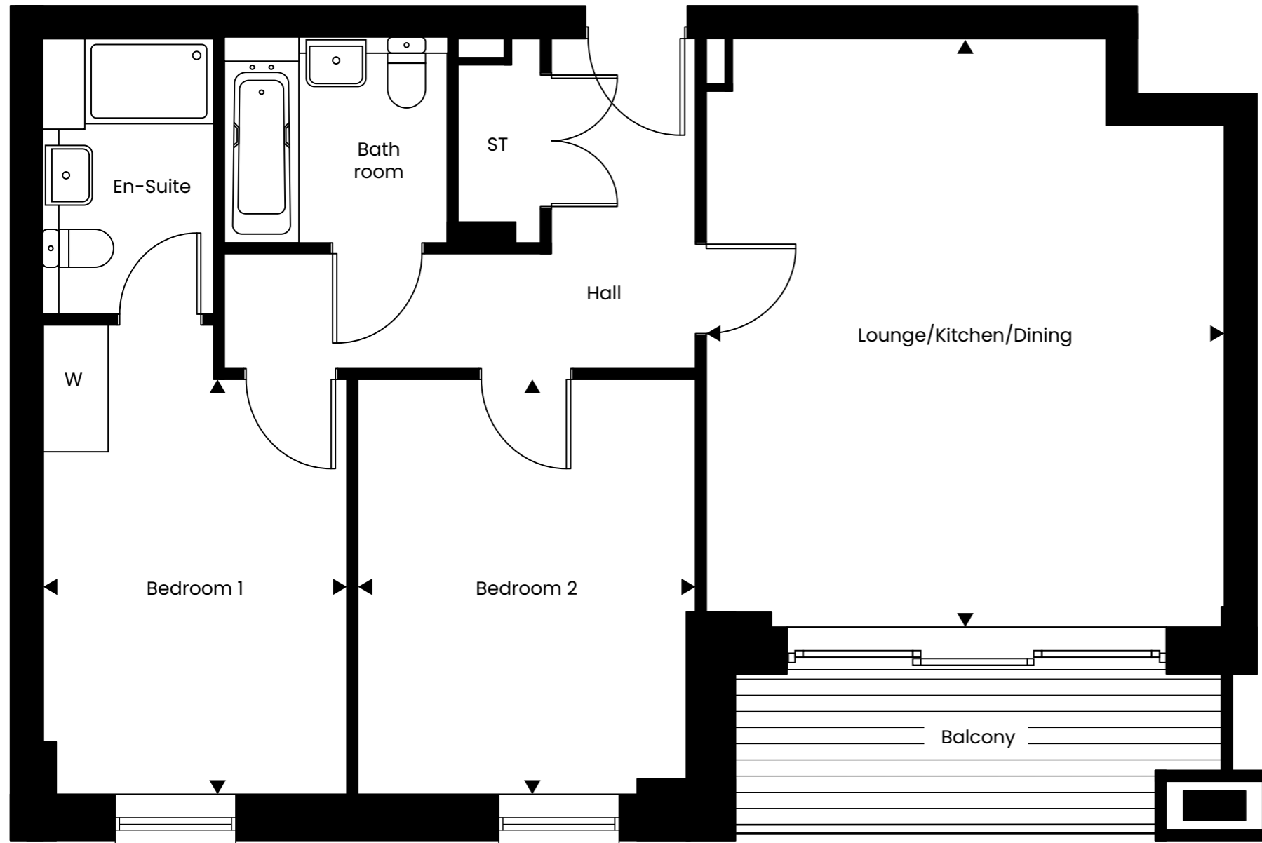
First Floor
