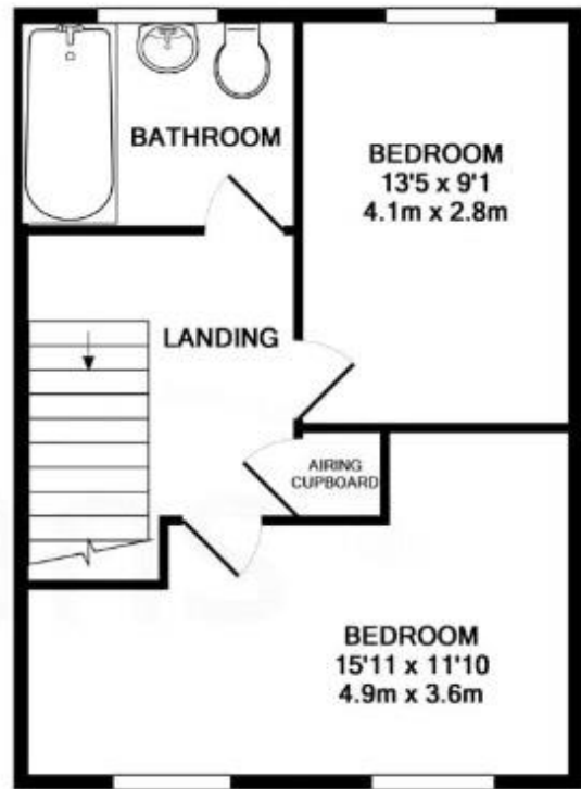
1ST FLOOR APPROX. FLOOR AREA 453 SQ.FT. (42.1 SQ.M.)
