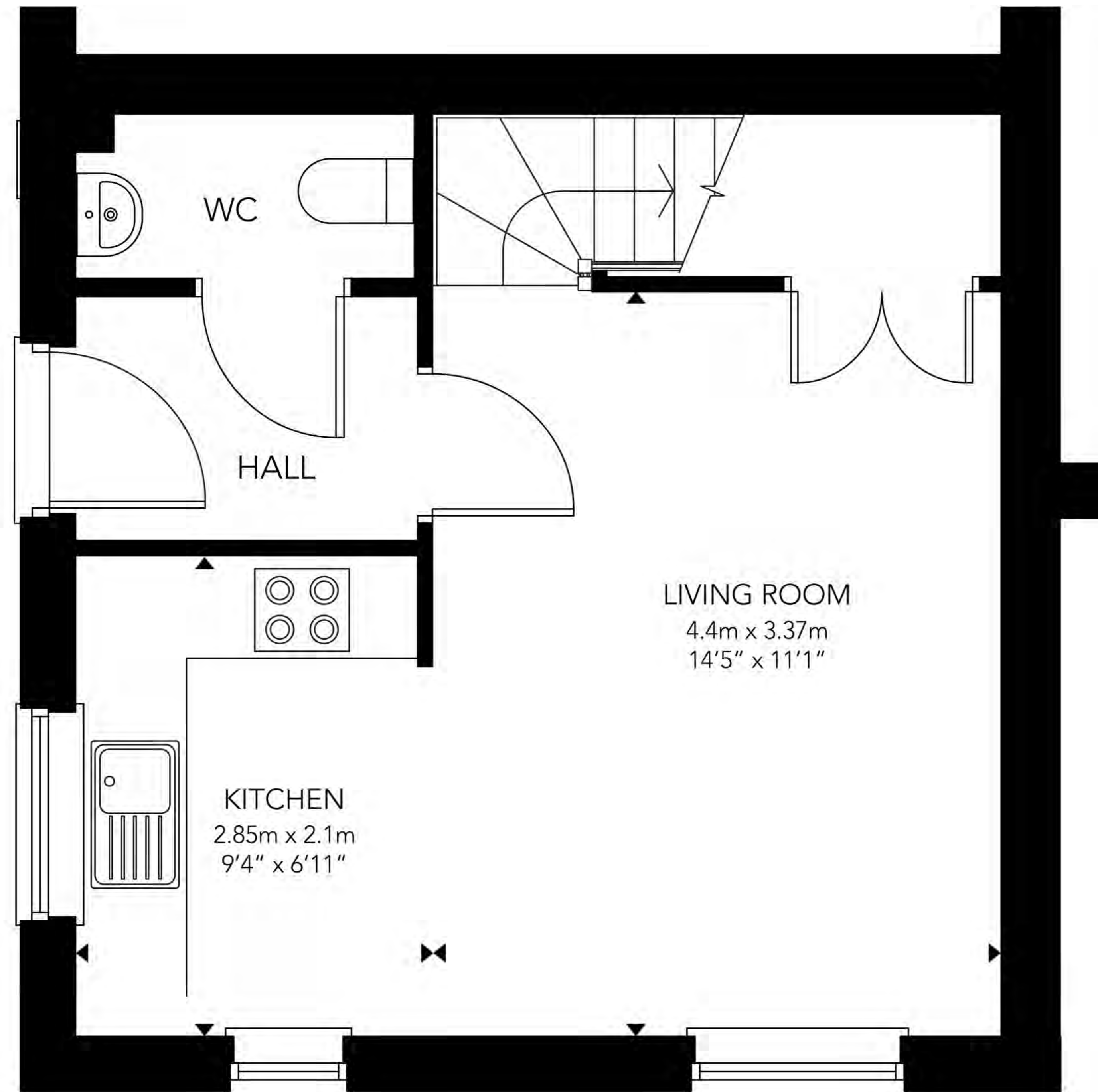
Ground Floor
