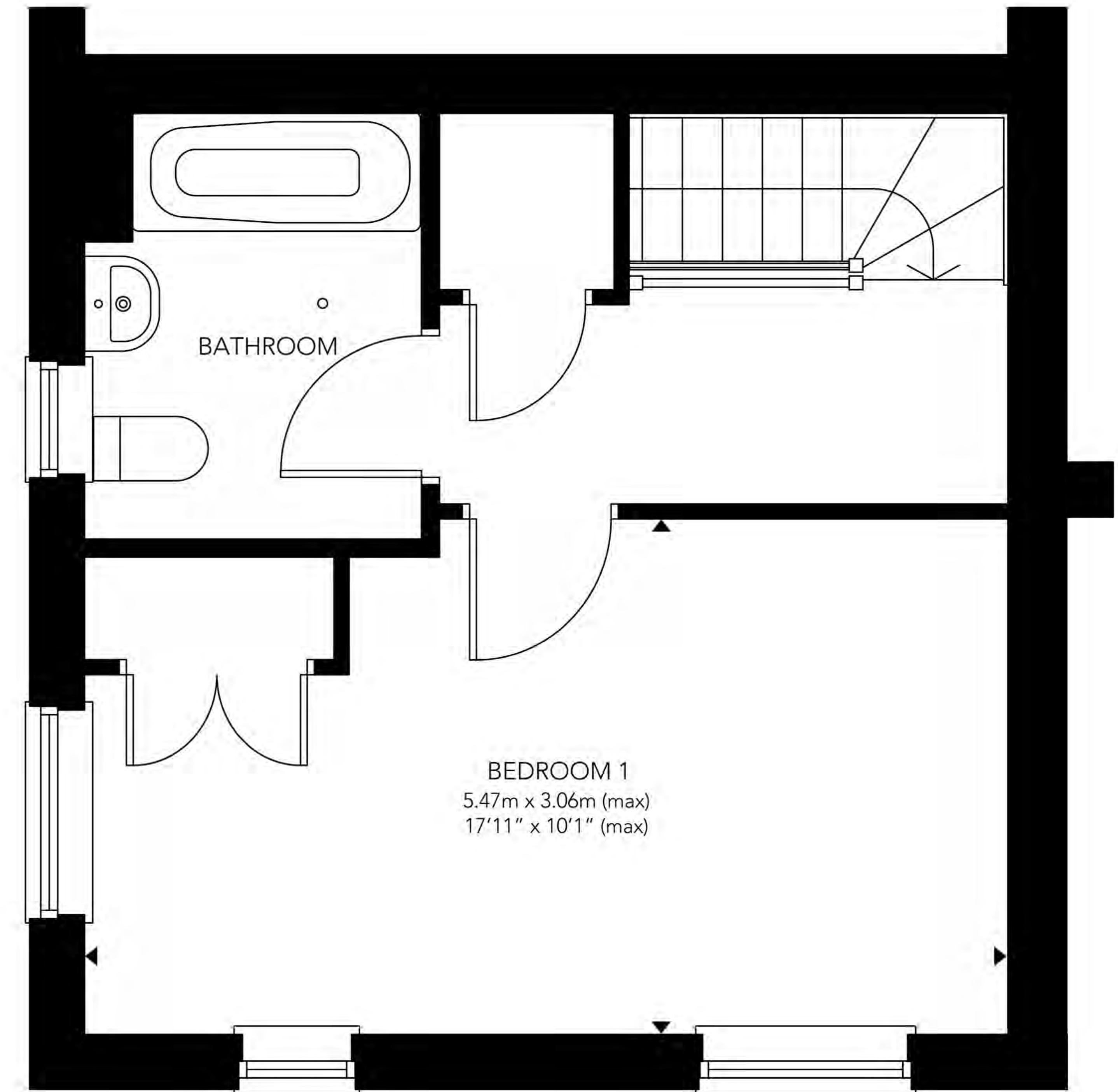
1st Floor
