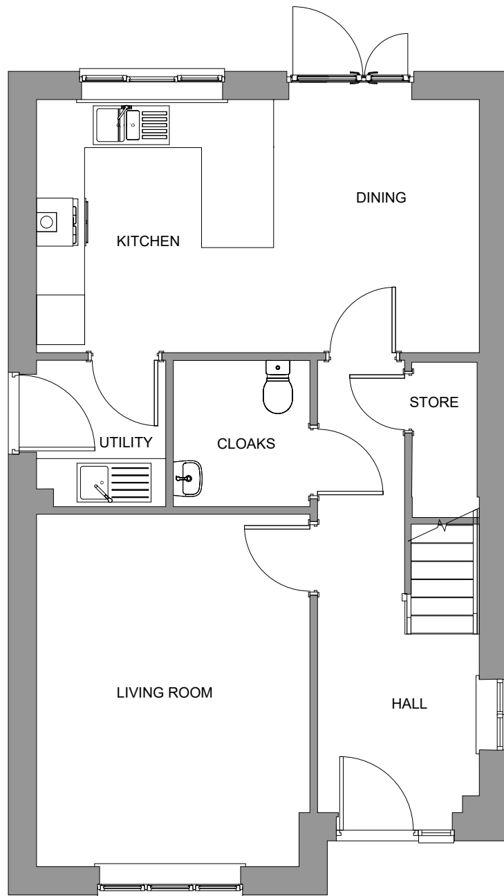
GROUND FLOOR
