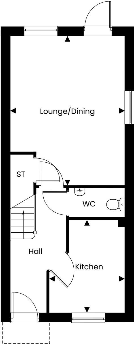
Ground Floor
