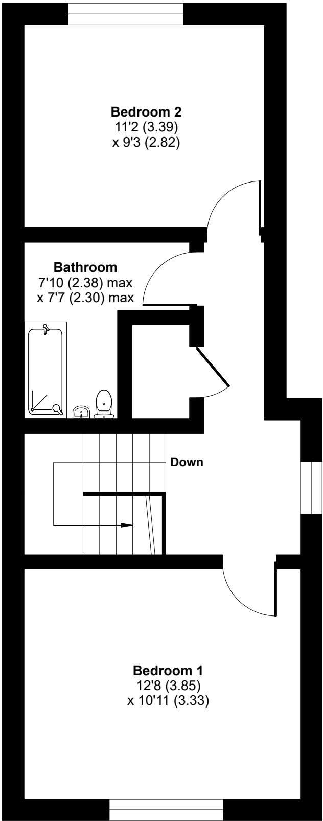
FIRST FLOOR
