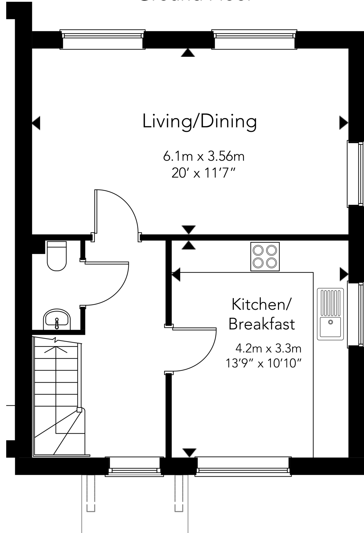
Ground Floor
