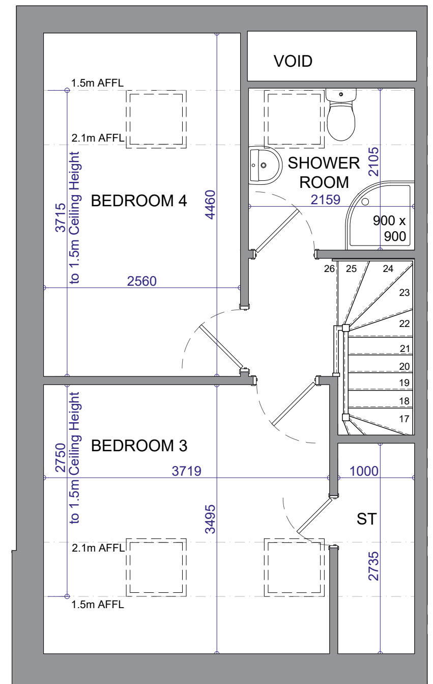
Second Floor
