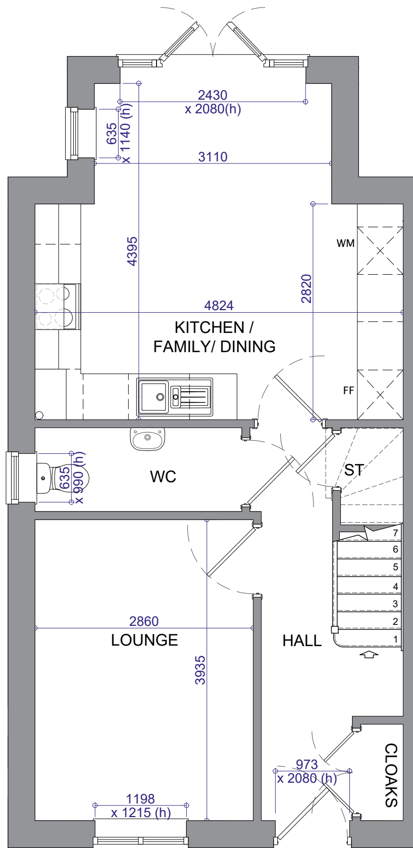
Ground Floor
