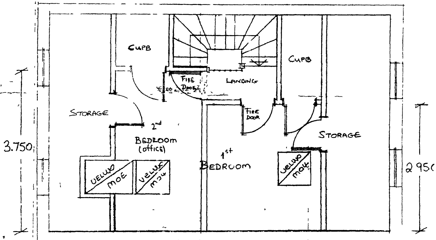
LOFT FLOOR PLAN
