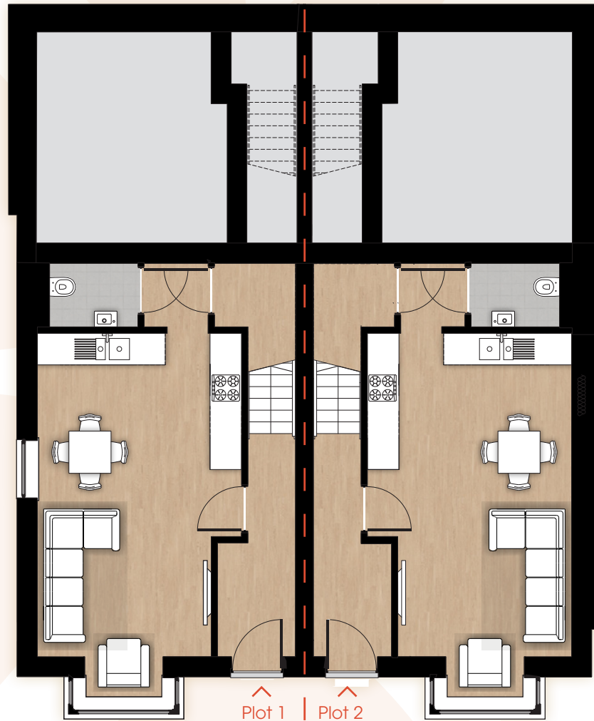
Ground Floor
